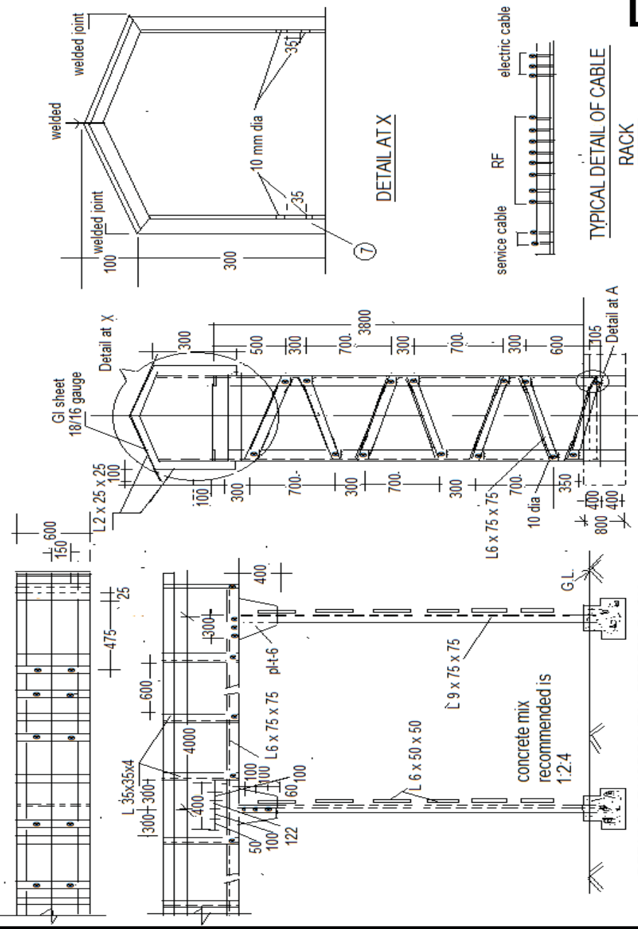
DETAILS OF HORIZONTAL FEEDER RACK
