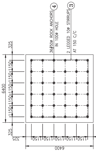
SECTION B-B PEDESTAL DETAILS-SOUTH SIDE
