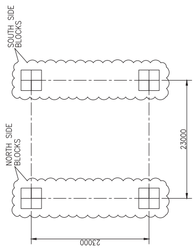
TYPICAL PLAN OF FOUNDATION
